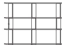
*Stock Size Jaunt 150 H107 shelf W1500 x D380 x H1065
